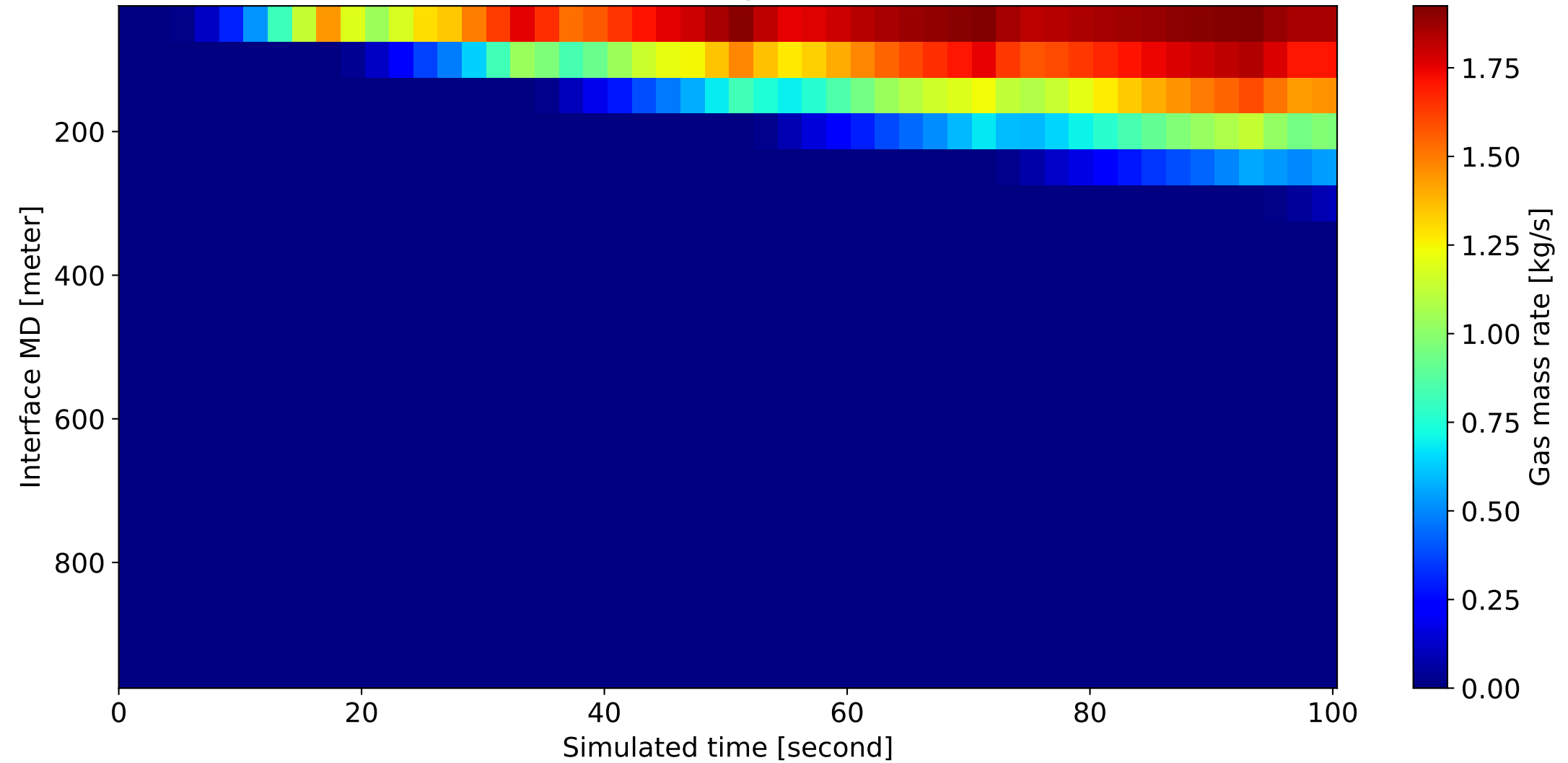
Gas mass rate profile along the wellbore over time
